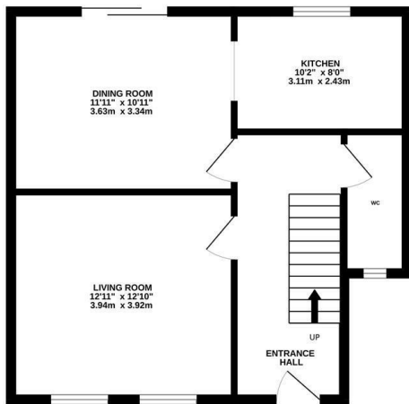
GROUND FLOOR 485 sq.ft. (45.1 sq.m.) approx.
