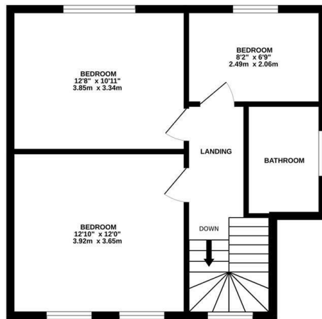
1ST FLOOR 485 sq.ft. (45.1 sq.m.) approx.
